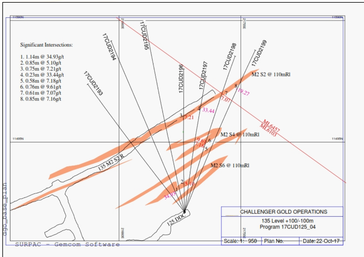
Figure 1: Phase 2 drilling targets - Plan view at 120mRL and shows bottom level of current Challenger development on the 135m RL level.
