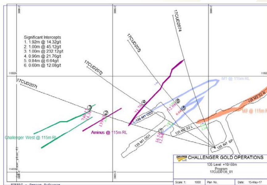
Figure 1: Phase 1 drilling targets (first 4 holes) - Plan view at 115mRL and shows bottom level of current Challenger development.
